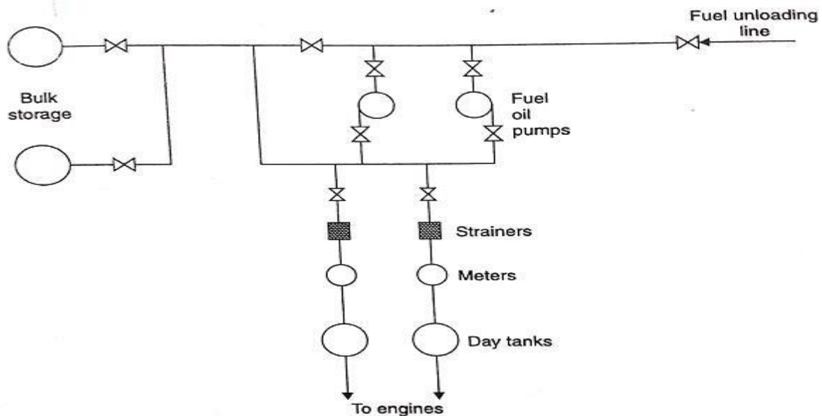
System of fuel storage for a diesel power plant.
