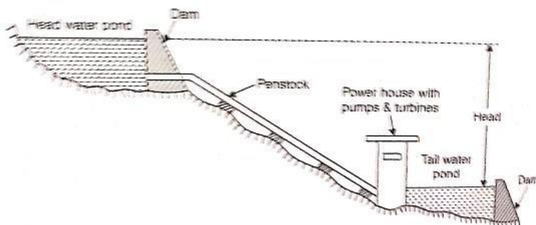
1. Pumped storage plant.
