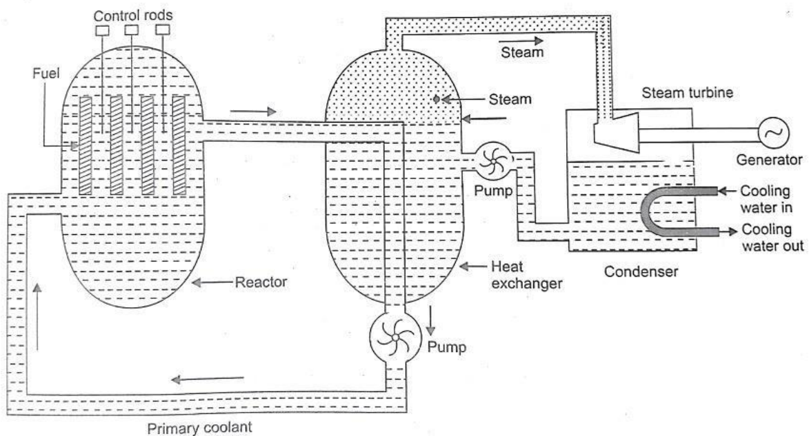
Pressurised water reaction (PWR)
