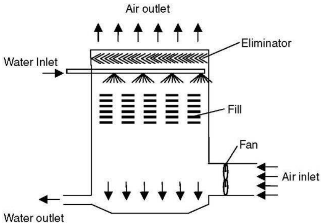
Fig : Forced draught cooling tower
