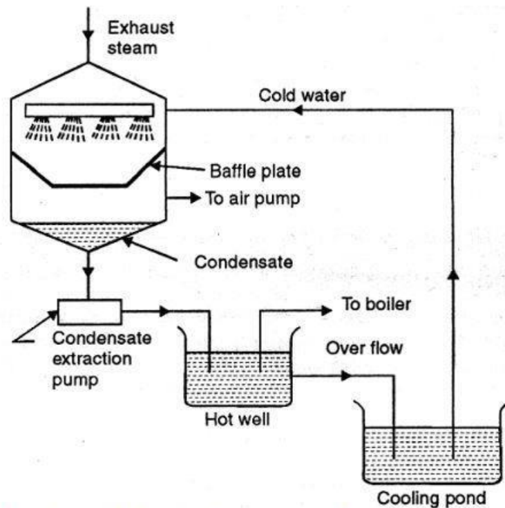
Fig. Parallel flow type condenser
