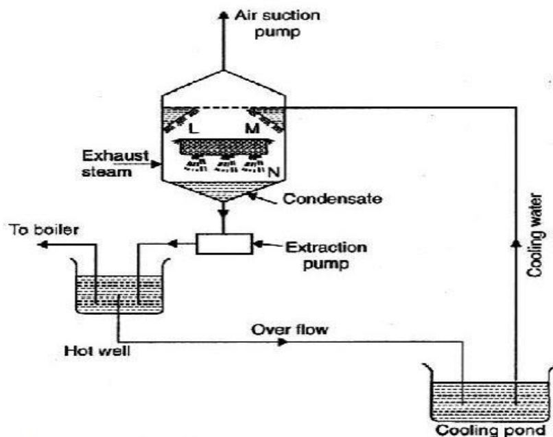
Fig. Low level counter flow type condenser
