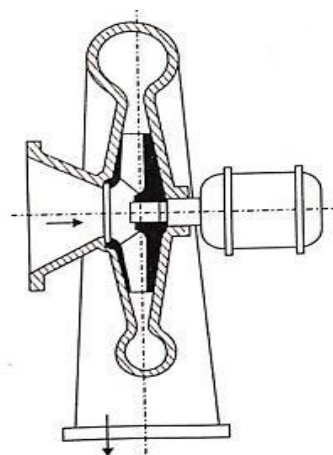
Single stage centrifugal compressor.
