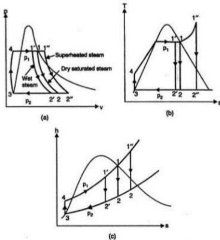
(a) p - v diagram ; (b) T - s diagram ; (c) h - s diagram for Rankine cycle.
