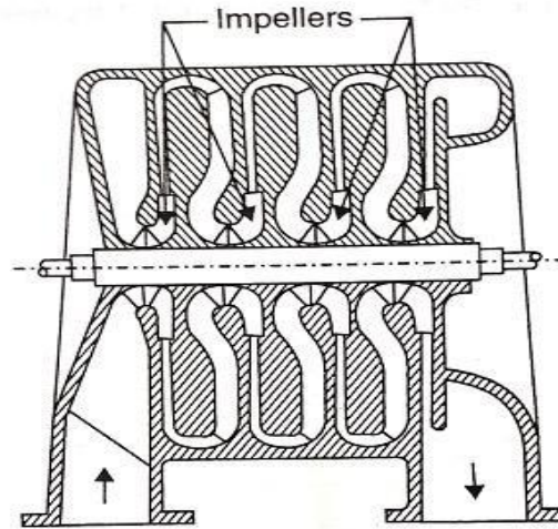
Multistage single flow axial compressor.
