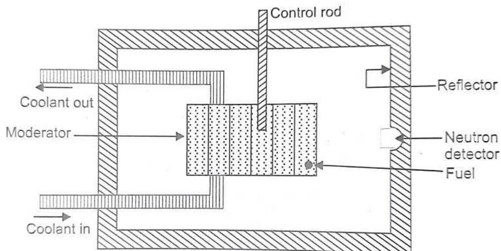
Fig. Reactor core
