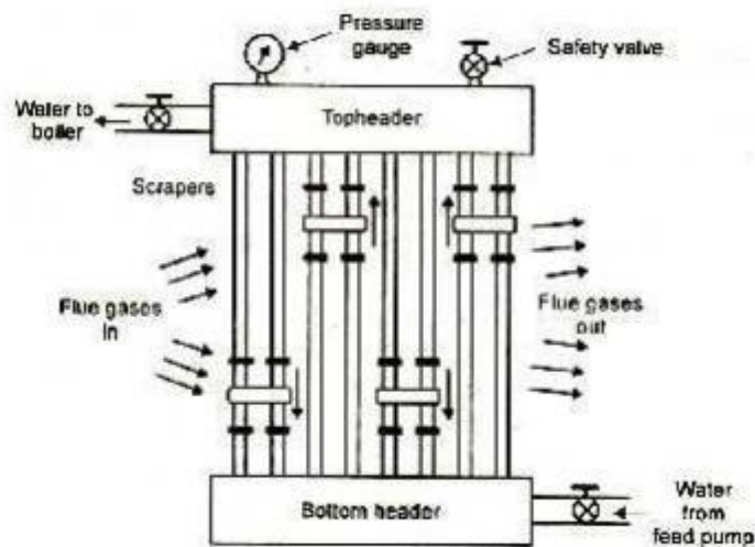
Fig. Economizer
