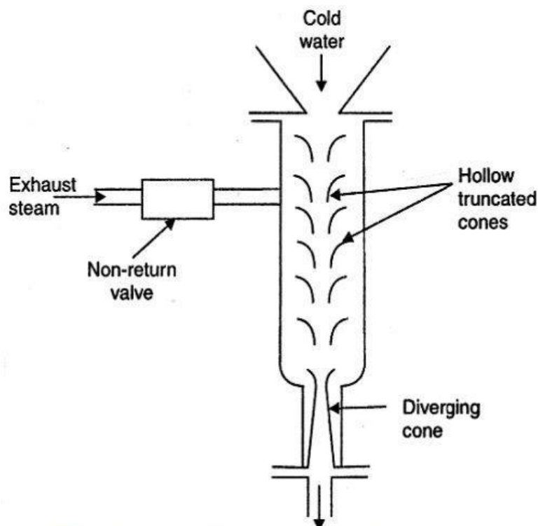
Fig. Ejector flow type condenser
