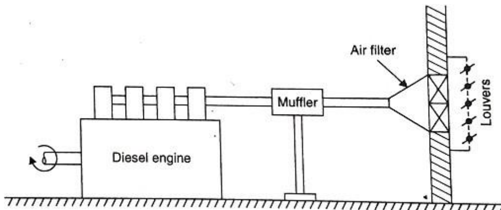
Fig. Air intake system.
