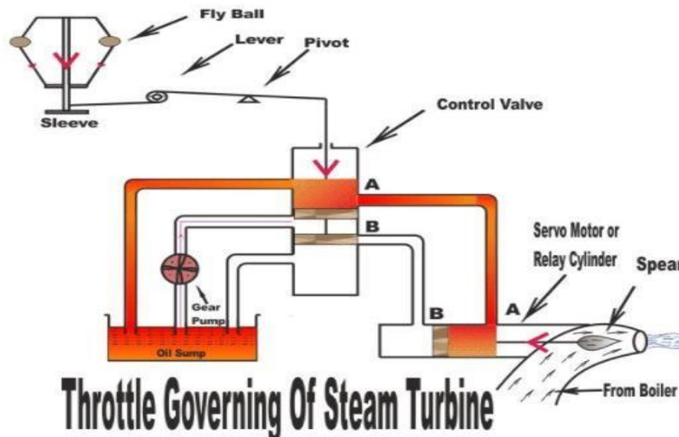
Fig : When Load increase on Turbine
