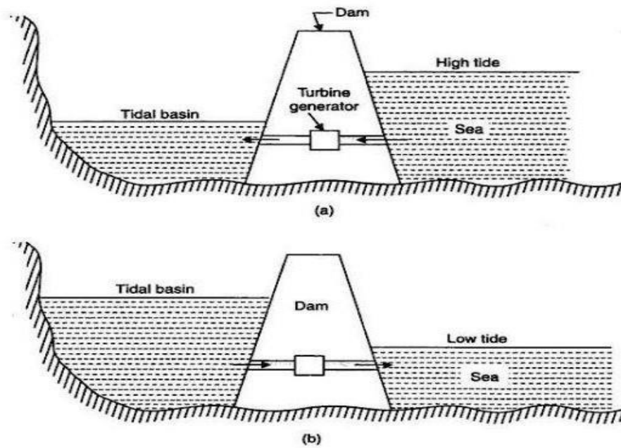
Fig. 1.1. Generation of power by tides.
