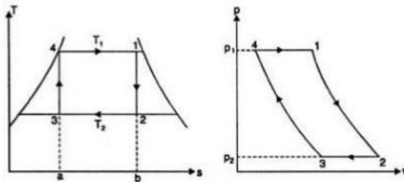
Carnot cycle on T-s and p-v diagrams.
