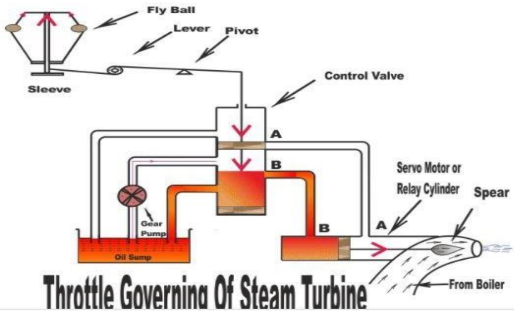
Fig : When Load Decrease on Turbine
