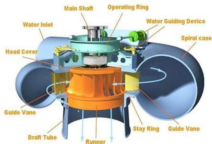
Francis Turbine
